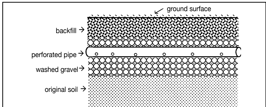
Figure 4 Septic Drainfield Courtesy—Washington State University
